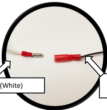
WIRED MAGNETIC INDUCTION MODULE
